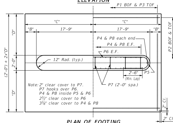
PLAN OF FOOTING
